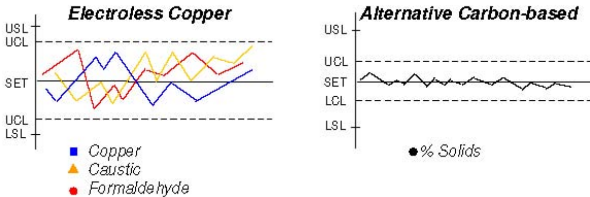
Figure 5 Process stability comparisons
