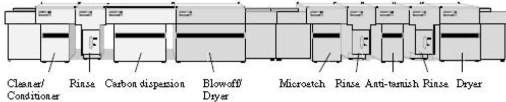
Figure 4 Horizontal Equipment Design
